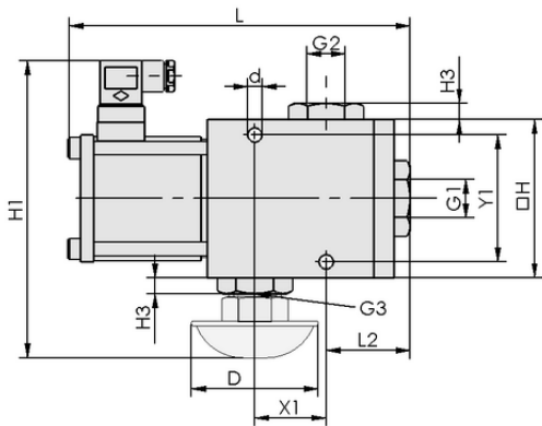
Design data EMVO 25 24V-DC 3/2 NC
