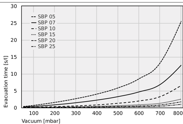
Evacuation time for various vacuum ranges [s/l]
