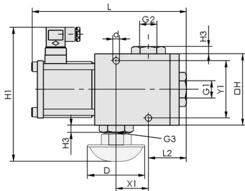
Design data EMVO 20 230V-AC 3/2 NC
