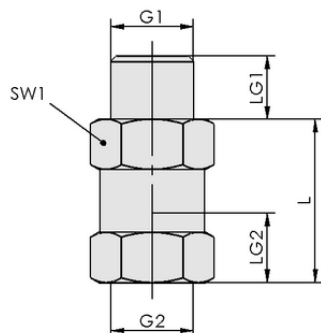
Design data SVK G1/8-IG
