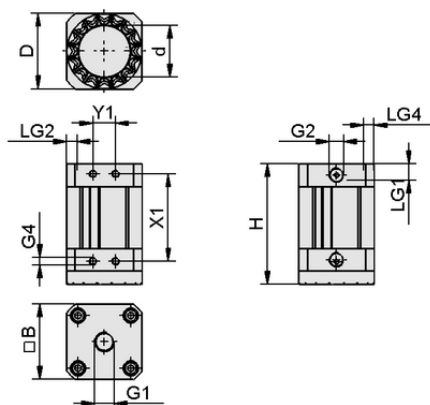
Design data SGM 40 G1/4-IG
