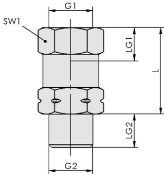
Design data SVKG G1/2-AG
