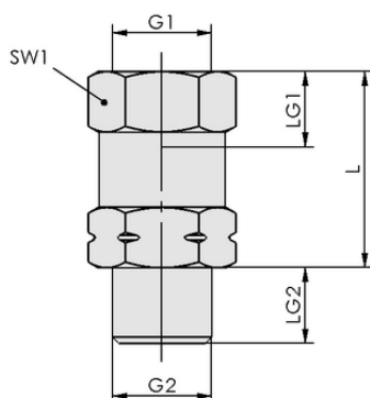
Design data SVKG G1/8-AG
