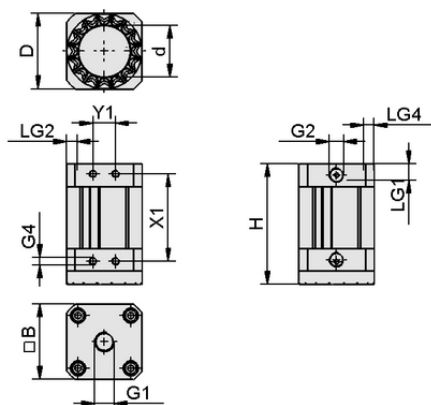
Design data SGM 30 G1/8-IG
